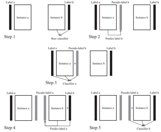
Figure 2: Five steps of model-reuse mechanism. Each white block represents the instance space. Each black strip refers to real labels and each gray strip stands for pseudo-label matrix predicted by learned classifiers.
