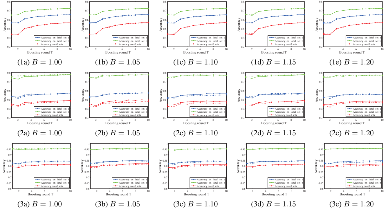
Figure 3: The five-fold cross-validation performance of DSML (mean) on Calligrapher-Font (sub-figures (1a) to (1e)), Brand-Type (sub-figures (2a) to (2e)), and Frequency-Gender (sub-figures (3a) to (3e)) datasets change with and without model-reuse mechanism when T increases with fixed value of B . The solid lines represent the performance with model-reuse mechanism, dotted lines otherwise.
